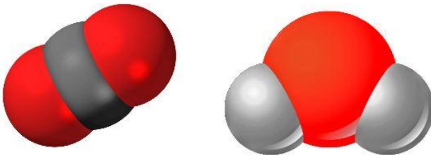
\text{CO}_2
