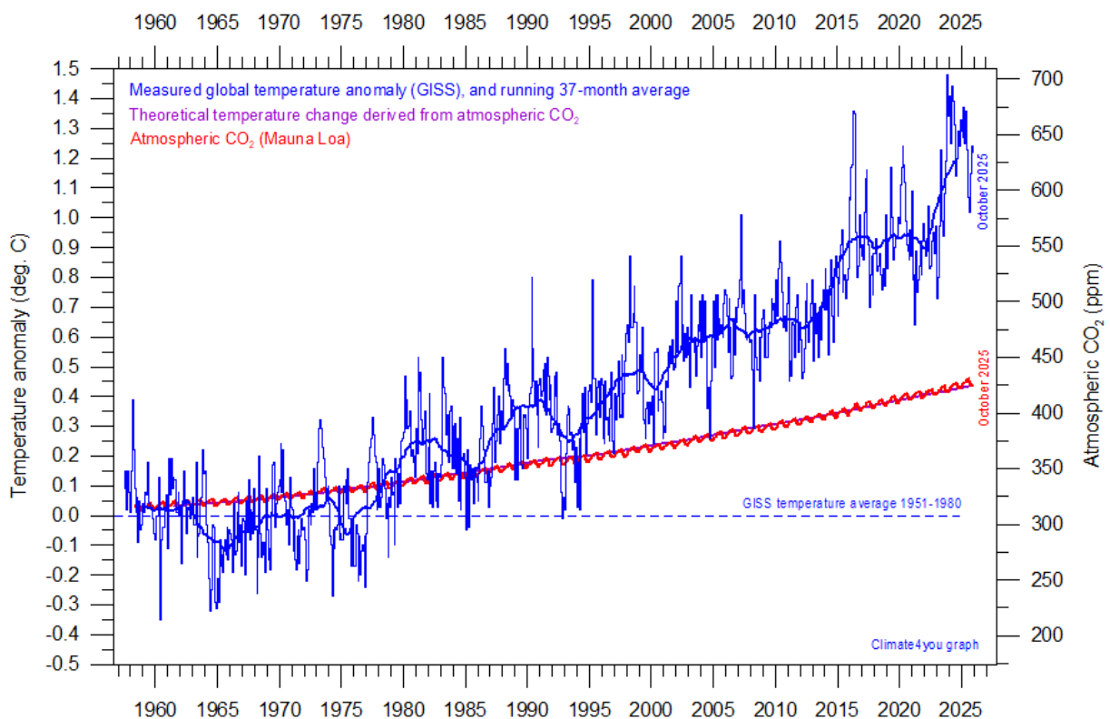
Temperature records versus atmospheric CO 2
